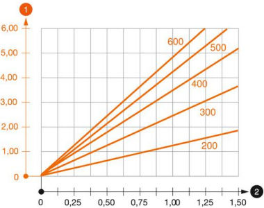
Load diagram, bracket type AS 15
