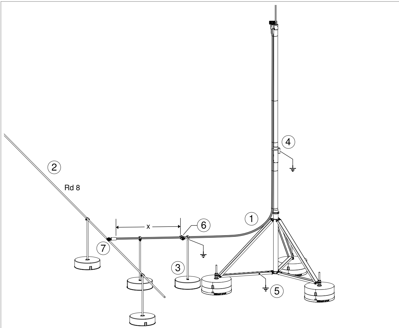
Fig. 62: isCon® conductor connected to stand-off ring conductor
