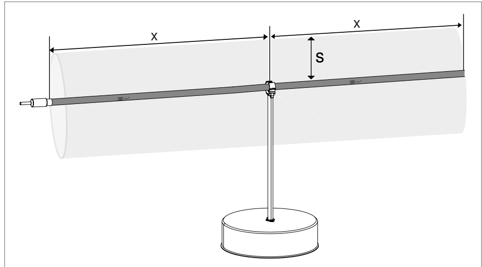
Fig. 56: Mounting variant for the isCon® conductor without potential connection
