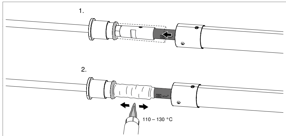
Fig. 30: Shrinking the heat-shrinkable sleeve
