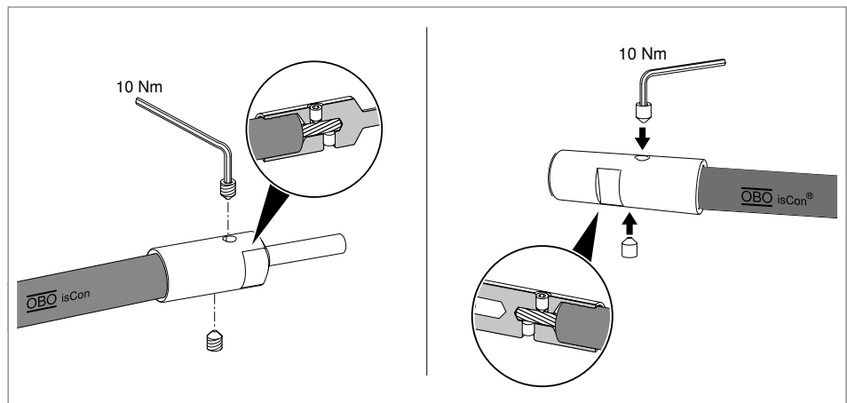
Fig. 25: Tightening the grub screws
