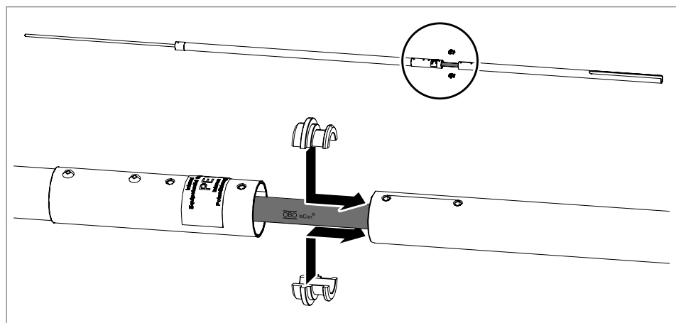
Fig. 31: Attaching the internal potential connection element
