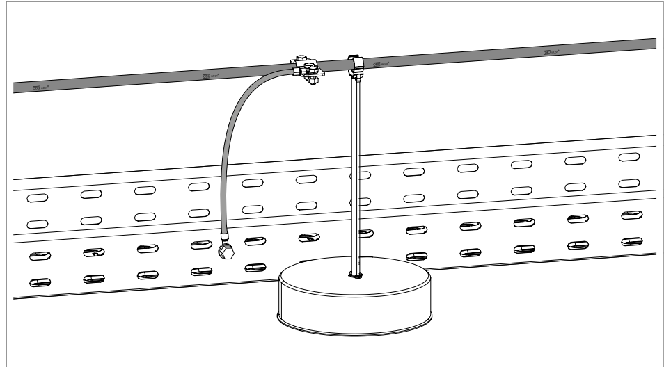
Fig. 58: Creating additional equipotential bonding
