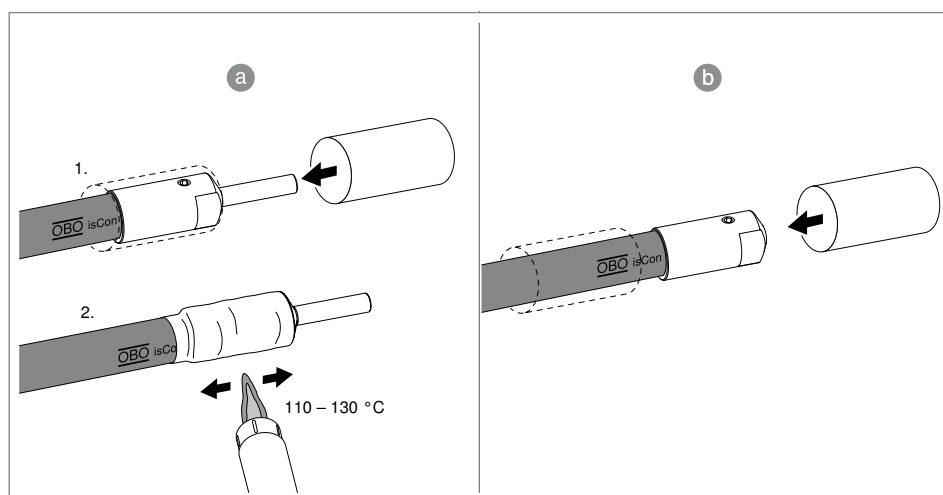
Fig. 26: Pull on heat-shrinkable sleeve
