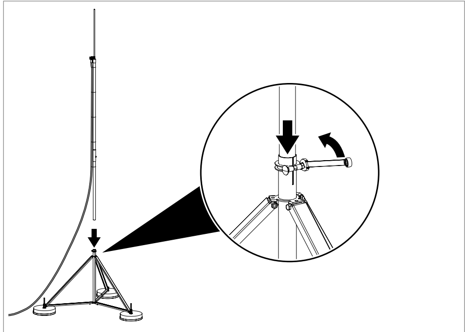
Fig. 48: Fixing the air-termination rod in the air-termination rod stand
